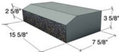
8x4x16 SOLID SLOPED SILL - SP1S, G1S OR SMO (SLOPED FACE G OR SMO)
