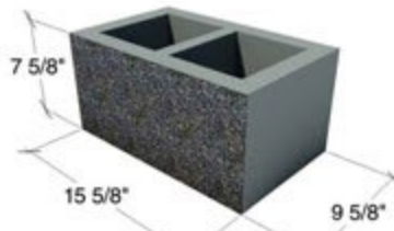
10x8x16 HOLLOW - SP1S, G1S, SMO
