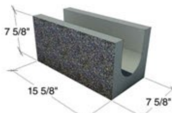
8x8x16 SOLID BOTTOM BB - SP1S, G1S, SMO
