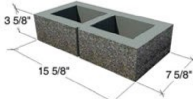
8x4x16 1S1F CORNER - SP1S, G1S, SMO
