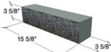
4x4x16 SOLID - SP1S, G1S, SMO
