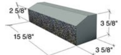
4x4x16 SOLID SLOPED SILL - SP1S, G1S OR SMO (SLOPED FACE G OR SMO)
