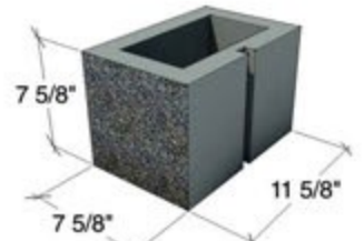
12x8x8 SASH - SP1S, G1S, SMO
