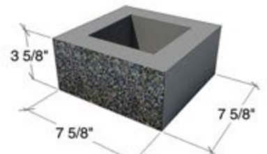
8x4x8 HALF - SP1S, G1S, SMO
