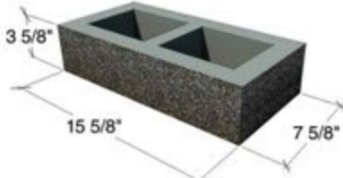
8x4x16 CORNER - SPC, G1S1E, SMO
