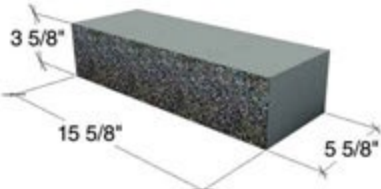
6x4x16 SOLID - SPC, G1S1E, SMO
