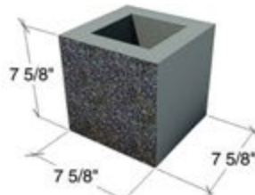
8x8x8 HALF - SP1S, G1S, SMO
