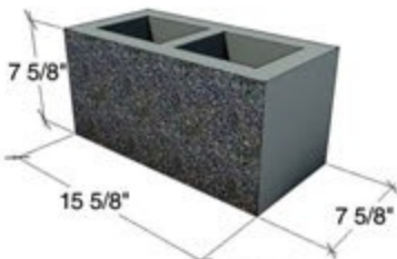
8x8x16 HOLLOW - SP1S, G1S, SMO
