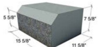
12x8x16 SOLID SLOPED SILL - SP1S, G1S OR SMO (SLOPED FACE G OR SMO)
