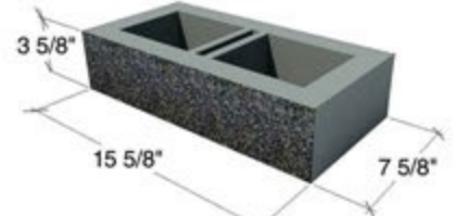
8x4x16 SPITTABLE - SPC, G1S1E, SMO
