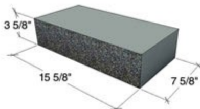
8x4x16 SOLID - SP1S, G1S, SMO
